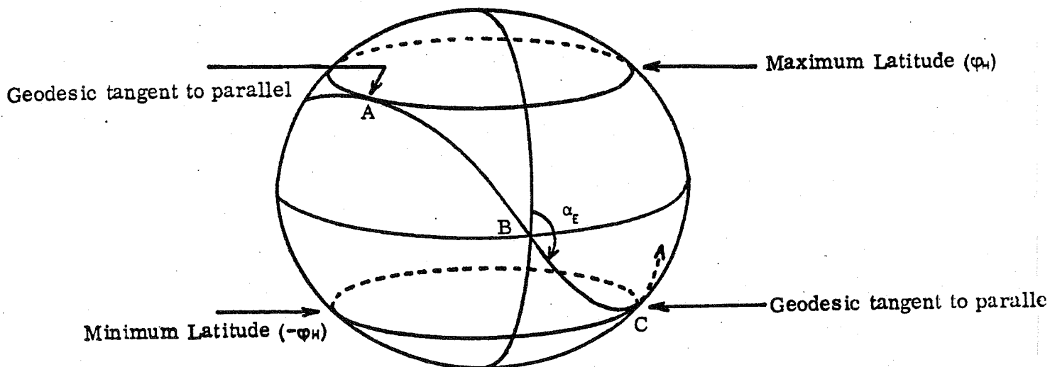
Figure 4.20 The Geodesic in a Continuous Form
