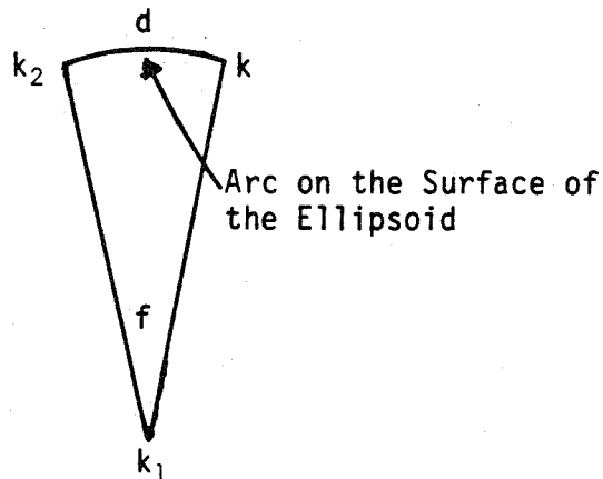
Figure 4.7 Linear Separation
