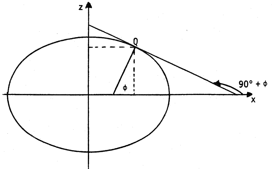
Figure 3.4 The Meridian Ellipse
