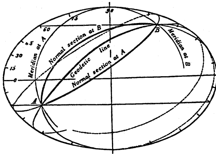
Figure 4.18 A Geodesic and Normal Section on a Highly Flattened ( f=1/3 ) Ellipsoid
