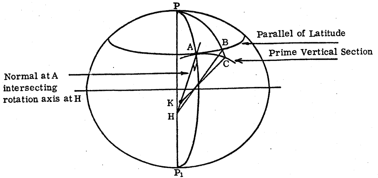
Figure 3.12 Geometric Derivation for N(A)
