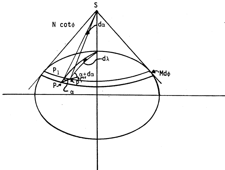
Figure 4.19 A Differential Figure on the Ellipsoid
