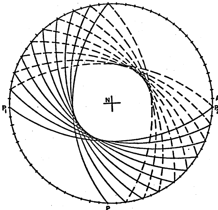
Figure 4.21 A View of a Continuous Geodesic from the North Pole Showing Consecutive Equator Crossings
