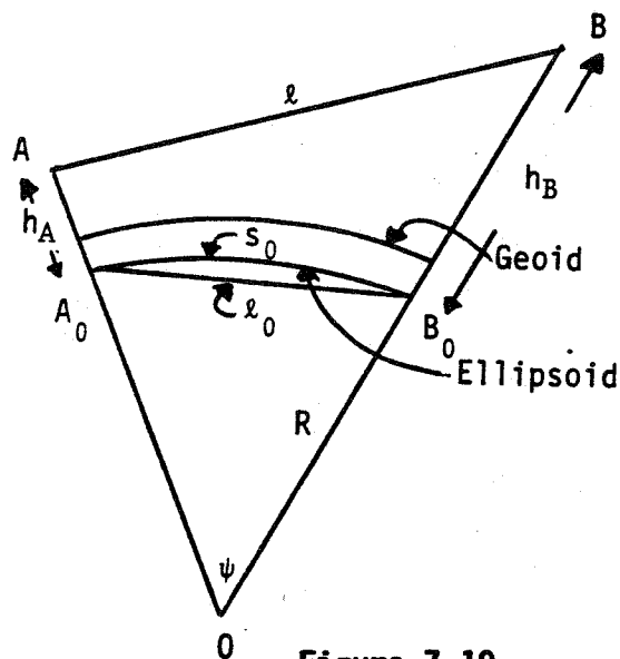
Figure 7.10 Reduction of Chord Distances to the Ellipsoid
