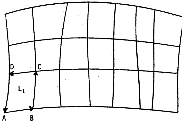
Figure 7.6 Astro-Geodetic Grid
