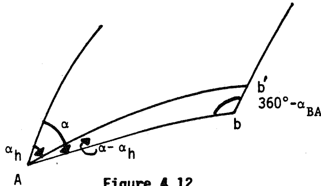
Figure 4.12 Small Triangle for Height Effect Determination
